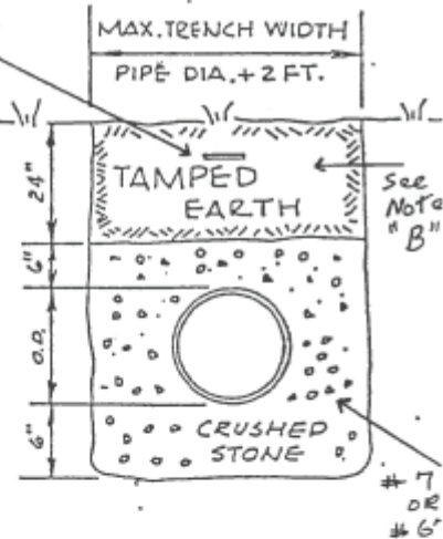
TYPICAL TRENCH SECTION NOT TO SCALE
