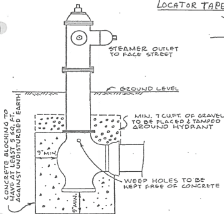
TYPICAL FIRE HYDRANT INSTALLATION
